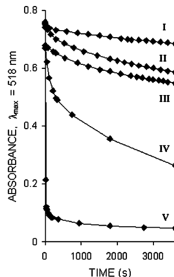
Figure 3. Continual absorbance decrease of ethanolic solution of \alpha,\alpha' -diphenyl- \beta -picrylhydrazyl (DPPH) radical (60 \mu M/L) in the presence of the antioxidants tested (33.3 \mu M/L) at \lambda_{\text{max}} = 518 nm.
